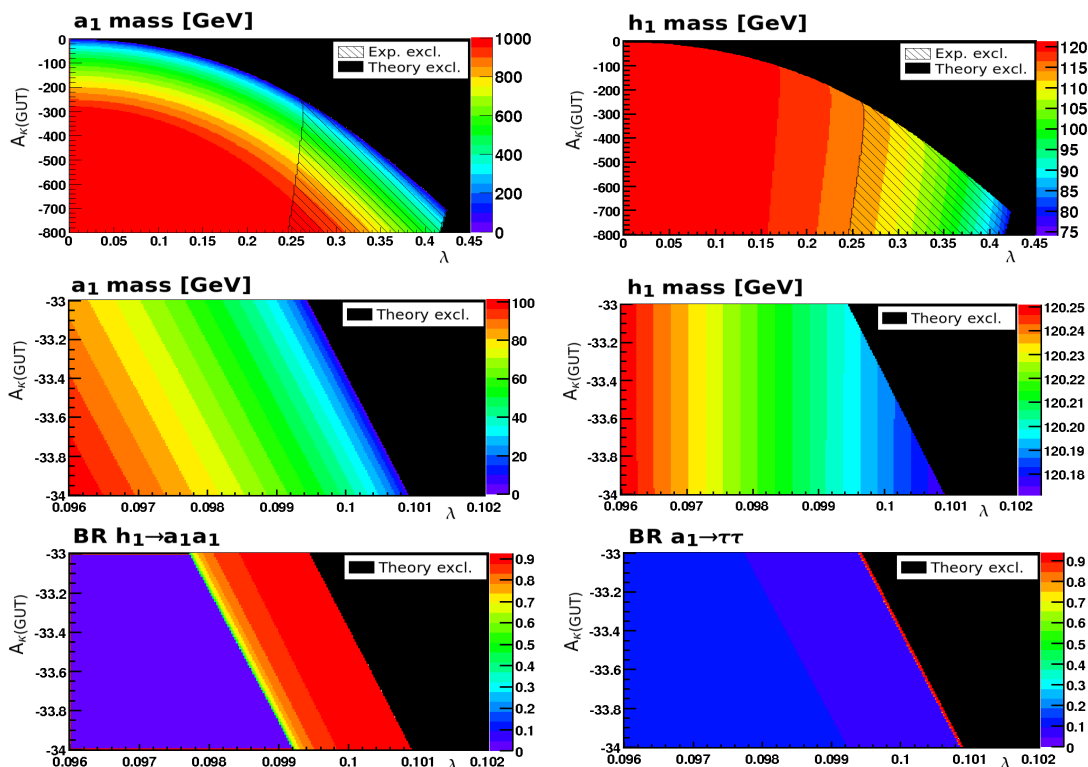
Figure 2: Scans in the [\lambda, A_\kappa] parameter space for the h_1^0, a_1^0 masses, and the branching ratios for the decay modes h_1^0 \rightarrow a_1^0 a_1^0 and a_1^0 \rightarrow \tau^+ \tau^- . The two upper frames include P1 to P3 while the remaining frames include only P1 and P2; other parameters as in figure 1.
