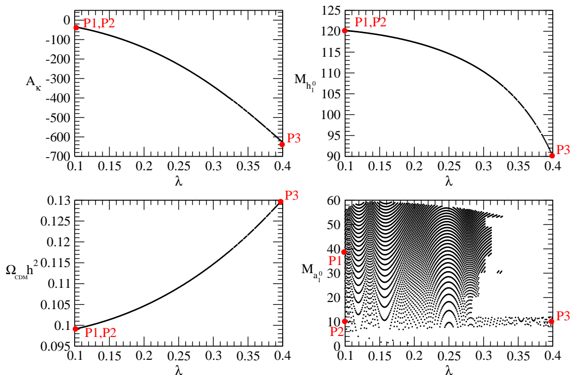
Figure 1: Allowed values of A_\kappa , M_{h_1^0} and M_{a_1^0} (in GeV) as well as \Omega_{\text{CDM}}h^2 as a function of \lambda . We take m_0 = 174 GeV, M_{1/2} = 500 GeV, A_0 = -1500 GeV and \tan\beta = 10 ; m_{\tilde{g}}^2 is determined from the electroweak symmetry breaking conditions.
